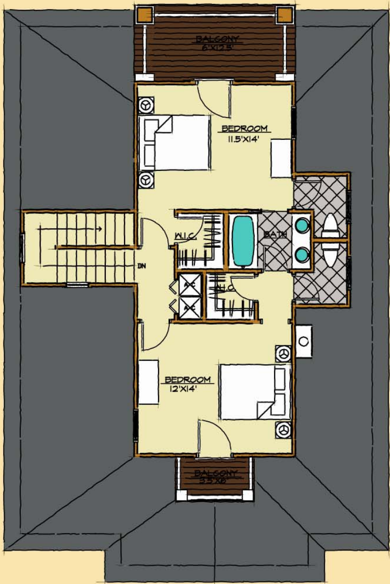
LUKE & BLUE'S CRAFTSMAN - SECOND FLOOR PLAN 563 S.E. H&C
